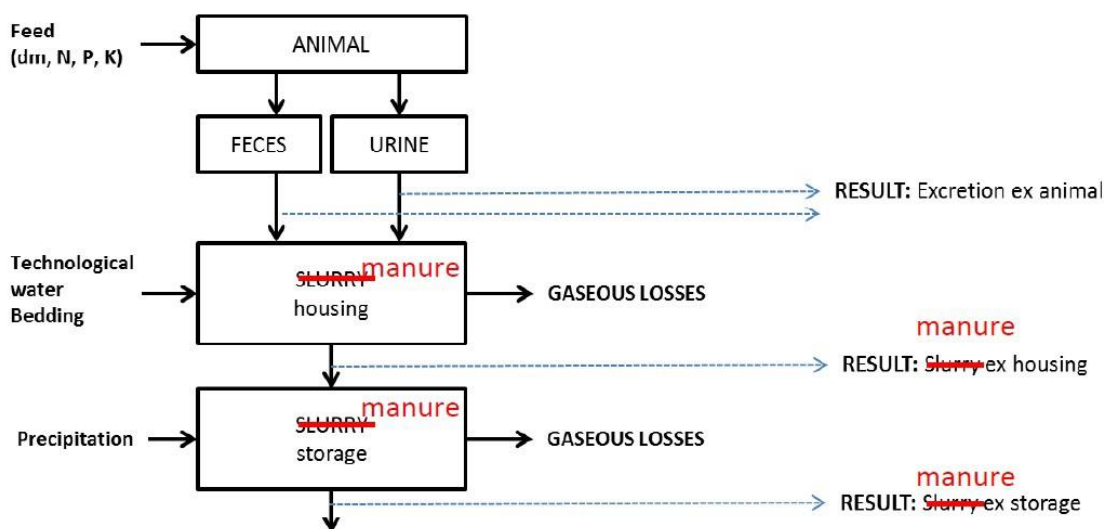
Figure 1. An example of the principle of manure mass balance calculation for slurry/liquid manure. The inputs to manure depend on the manure type and practices and structures of animal housing and manure storage.
